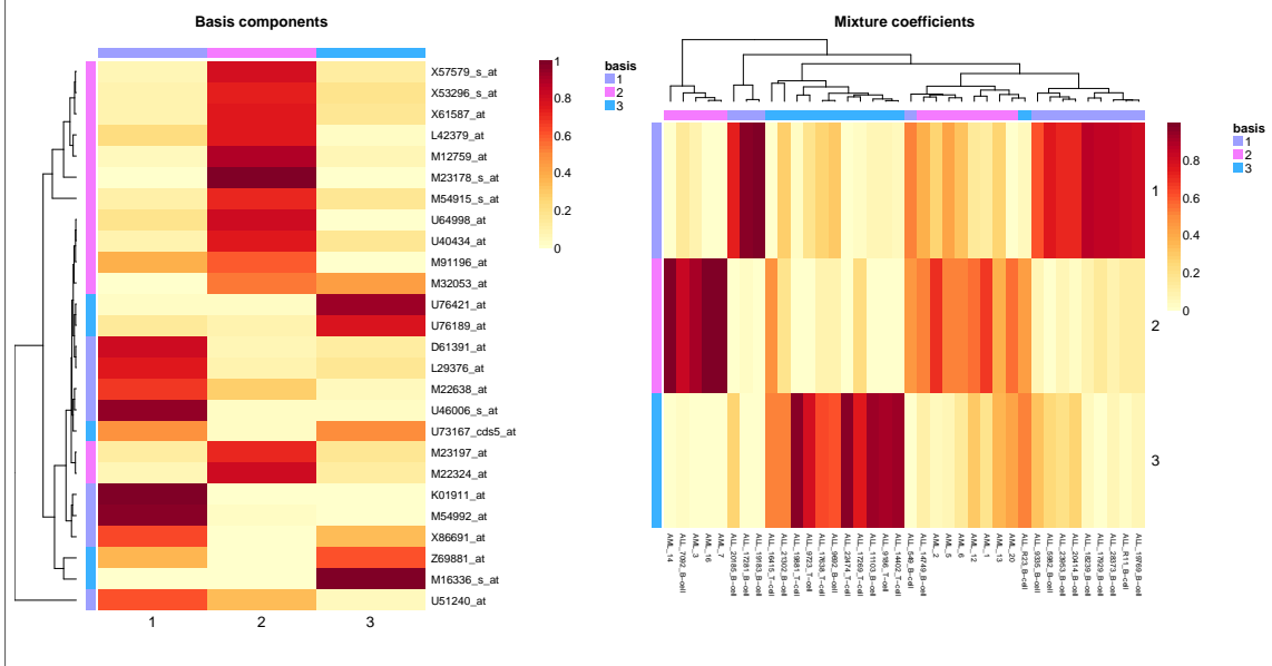
Figure 5: Heatmap of the basis and the mixture coefficient matrices. The rows of the basis matrix were selected using the default feature selection method – described in (Kim et al. 2007).
