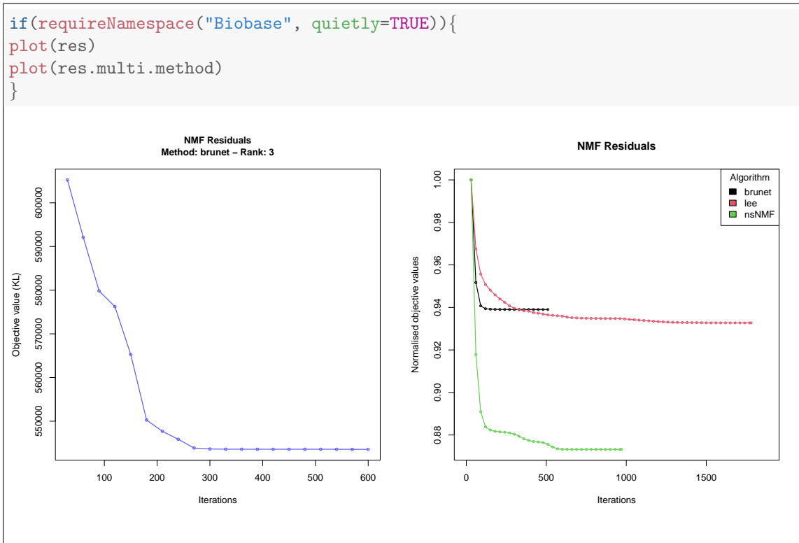
Figure 4: Error track for a single NMF run (left) and multiple method runs (right)
