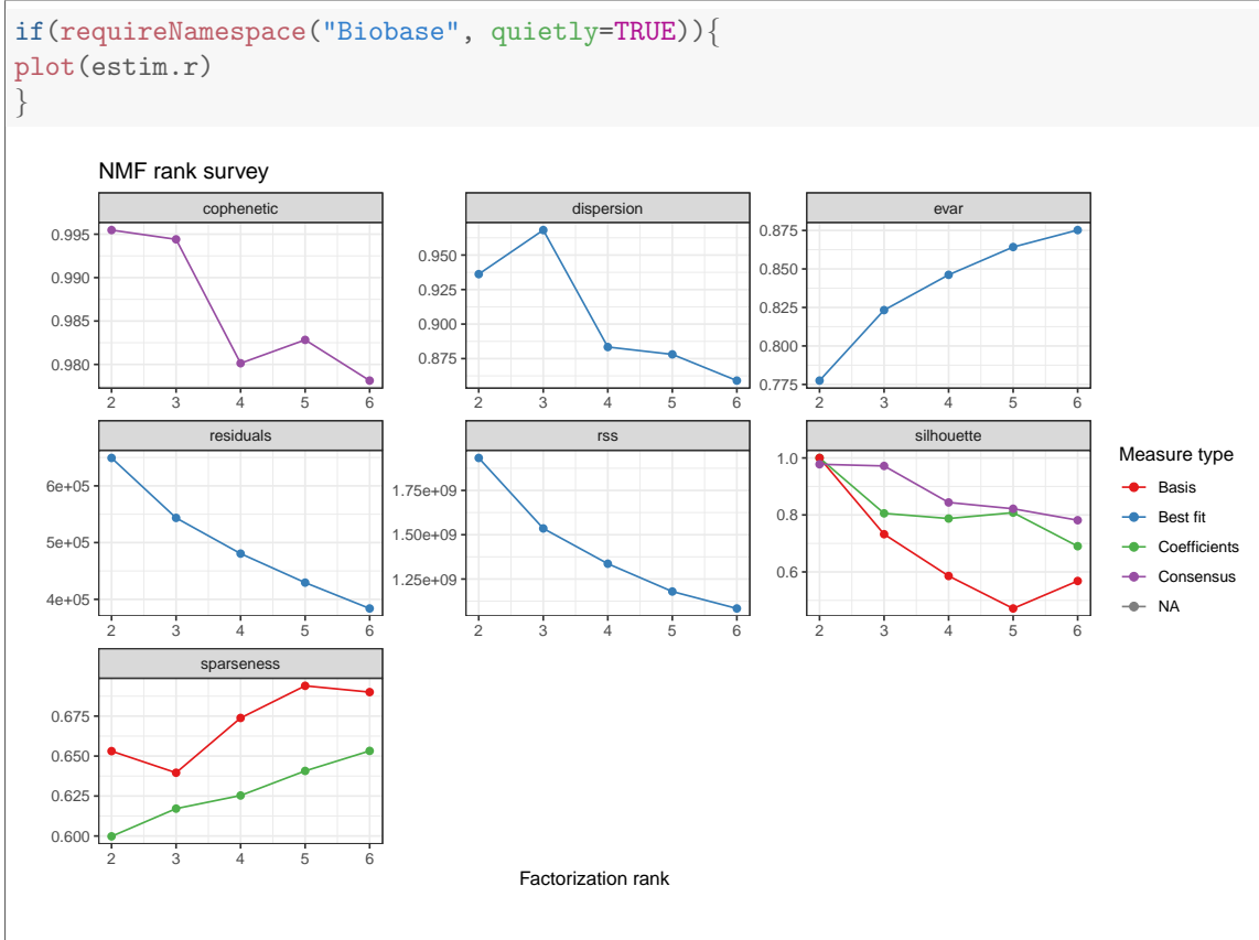
Figure 1: Estimation of the rank: Quality measures computed from 10 runs for each value of r .
